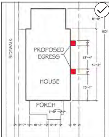
19. Locate a new basement egress window to be as inconspicuous as possible.
